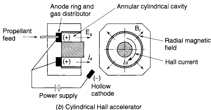
FIGURE 19–10. Linear and cylindrical Hall accelerator configurations showing how an applied axial field results in a transverse current that accelerates the plasma. The Hall current peaks when the external resistance is absent (i.e., shorted). The presence of any significant axial current density j_x represents an inefficiency in Hall devices.
