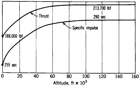
FIGURE 2-2. Altitude performance of RS 27 liquid propellant rocket engine used in early versions of the Delta launch vehicle.
